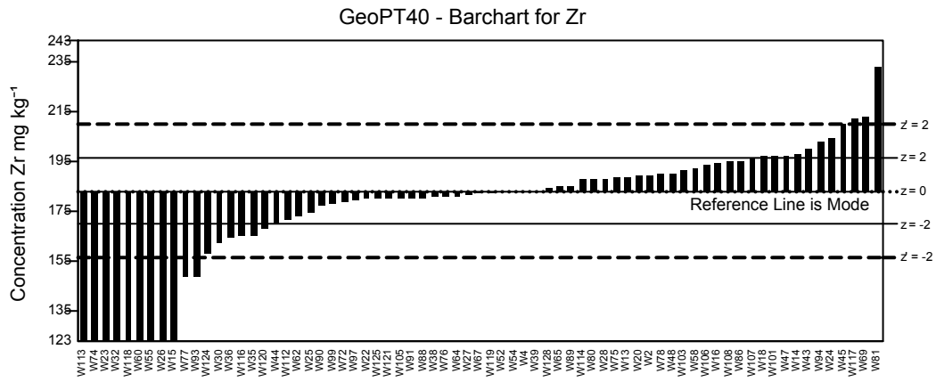
Figure 1: GeoPT40 - Silty marine shale, ShWYO-1. Data distribution charts for elements for which values were assigned or provisional values given for guidance. Horizontal lines show the limits for -2 < z < 2 for pure geochemistry labs (solid lines) and -2 < z' < 2 for applied geochemistry labs (pecked lines).
