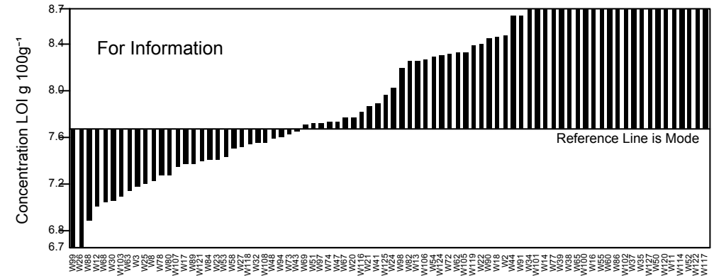
GeoPT40 - Barchart for B
