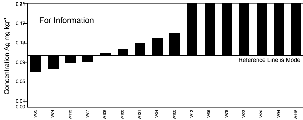
GeoPT40 - Barchart for Ag
