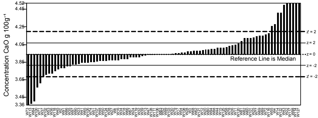
GeoPT40 - Barchart for CaO
