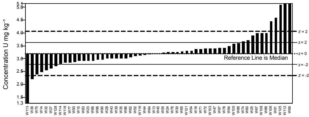
GeoPT40 - Barchart for W
