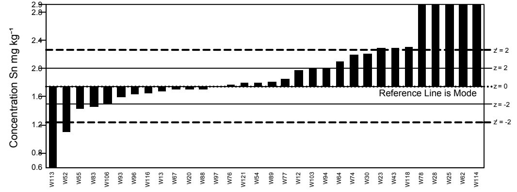
GeoPT40 - Barchart for Sn
