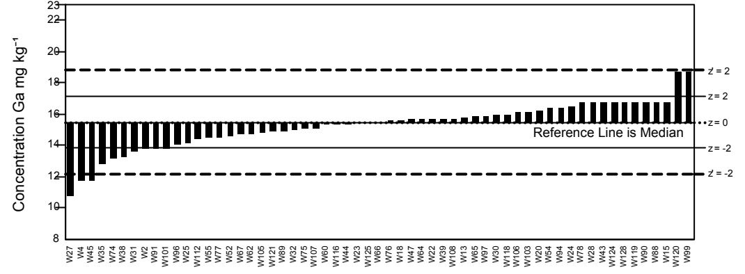
GeoPT40 - Barchart for Ga
