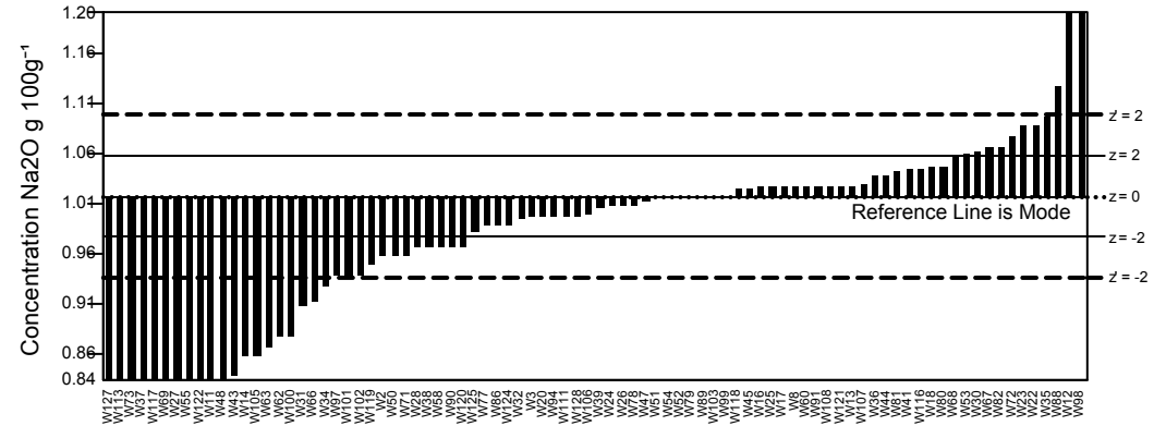
GeoPT40 - Barchart for Na2O
