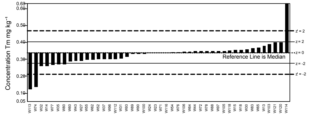
GeoPT40 - Barchart for Tm
