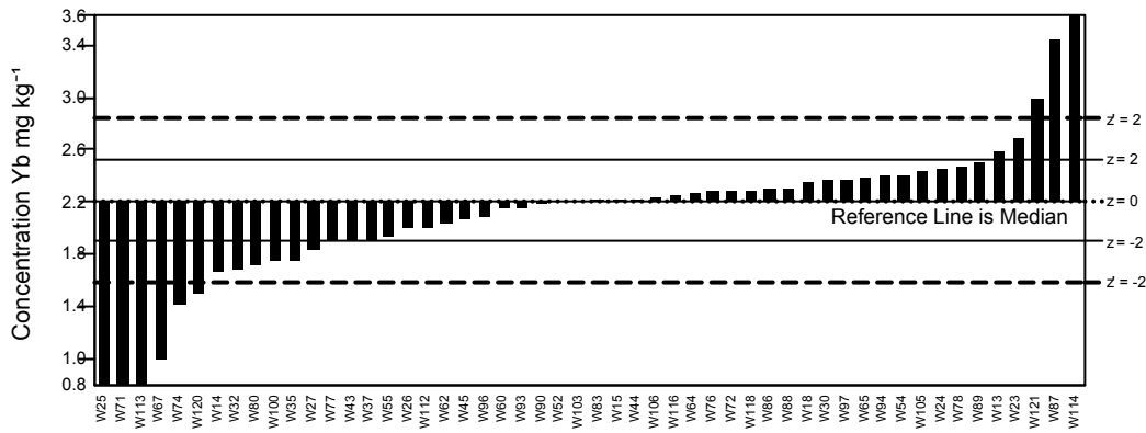
GeoPT40 - Barchart for Yb
