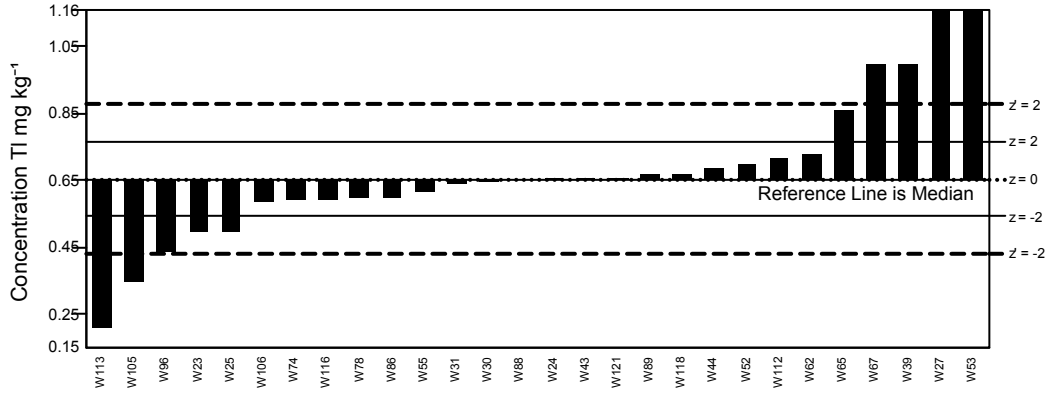
GeoPT40 - Barchart for Tl
