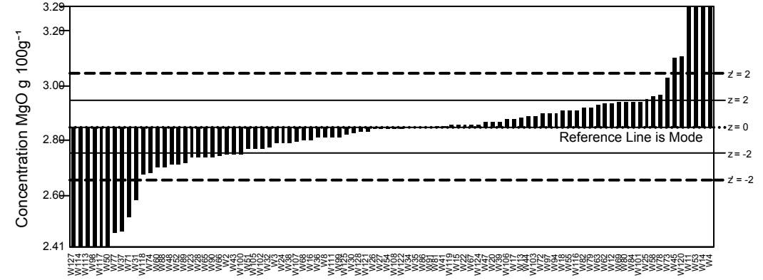
GeoPT40 - Barchart for MgO
