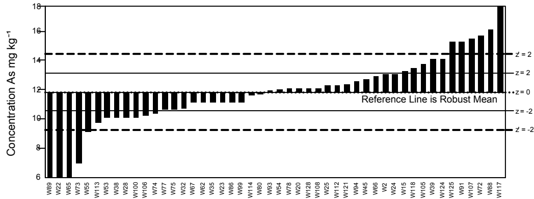
GeoPT40 - Barchart for As
