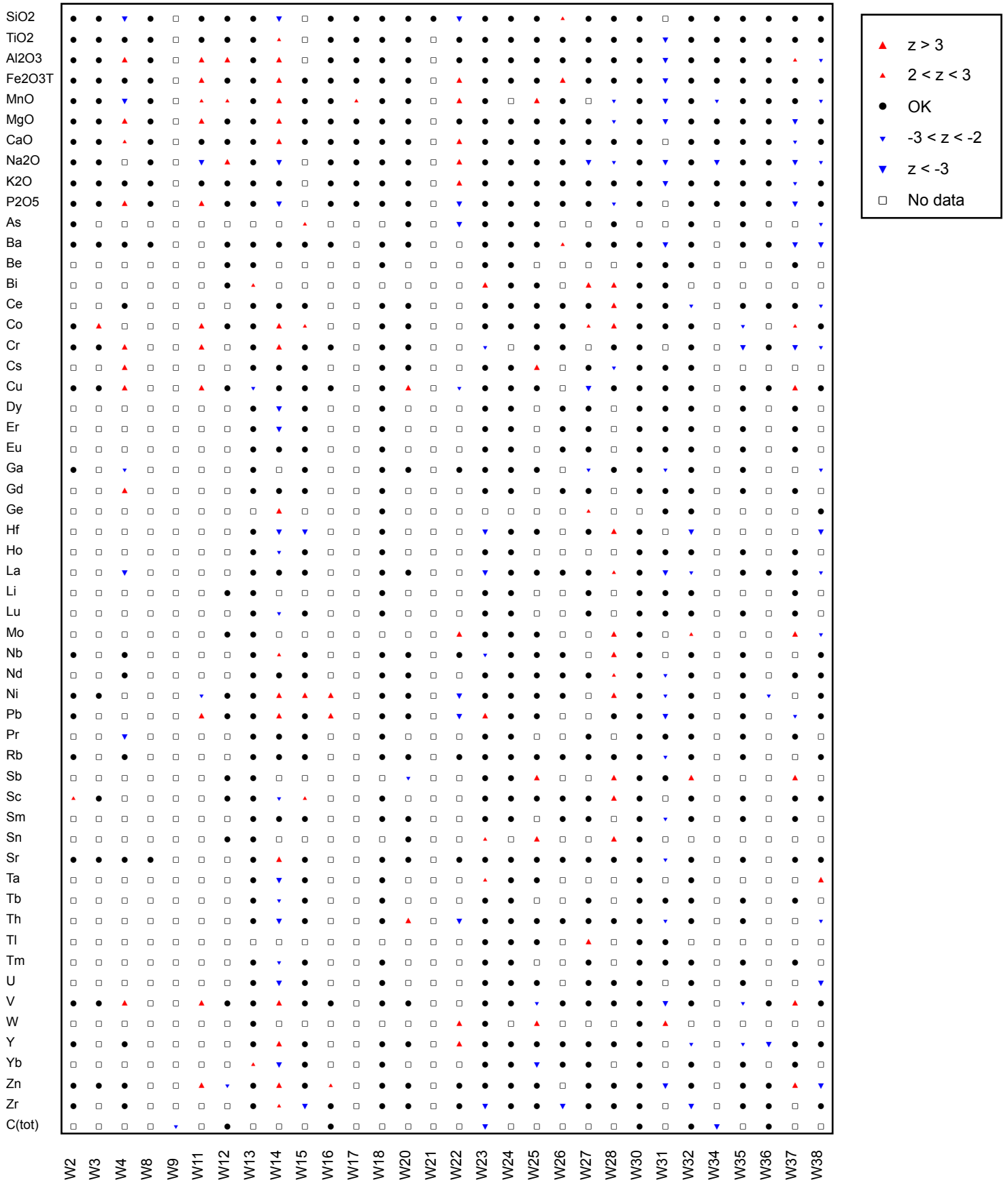
Figure 3: GeoPT40 - Silty marine shale, ShWYO-1. Multiple z-score charts for laboratories participating in the GeoPT40 round. Symbols indicate whether or not an elemental result complies with the -2 < z < +2 criteria (see key).
