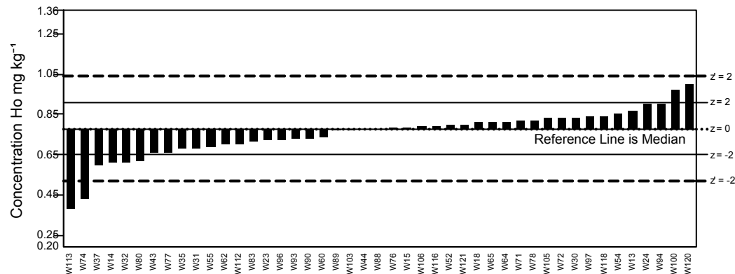
GeoPT40 - Barchart for Ho
