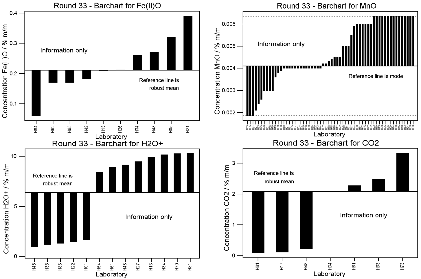
Figure 2.1: GeoPT33 – Ball clay, DBC-1. Data distribution charts for information only for elements for which values could not be assigned.
