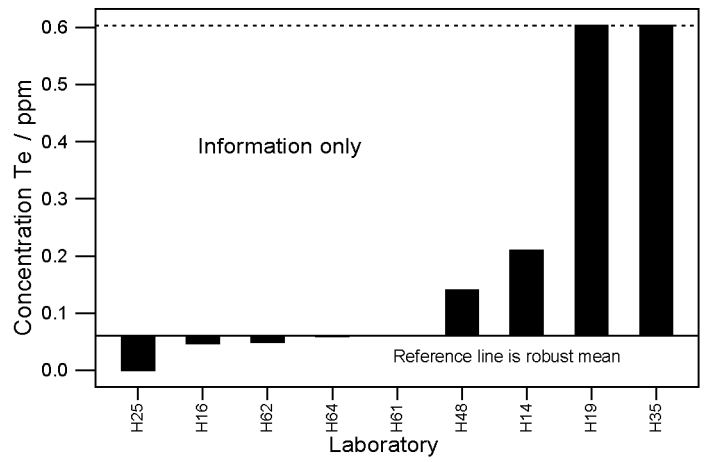
Figure 2.2: GeoPT33 – Ball clay, DBC-1. Data distribution charts for information only for elements for which values could not be assigned.
