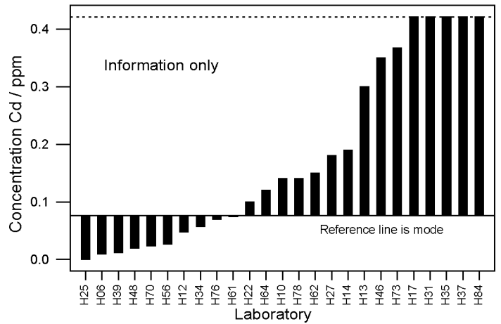
Round 33 - Barchart for In
