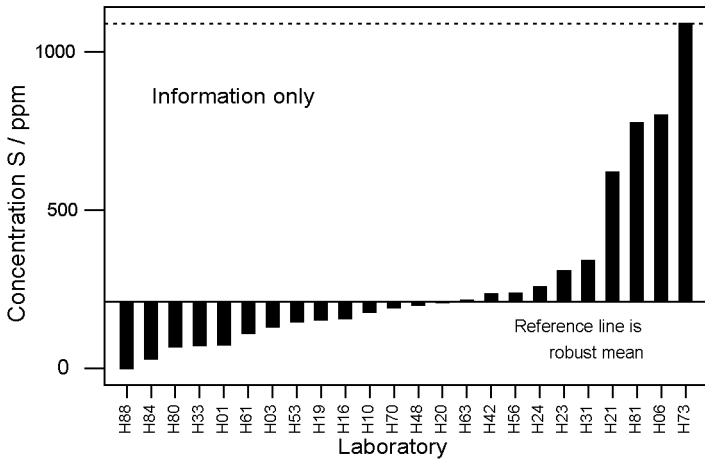
Figure 2.2: GeoPT33 – Ball clay, DBC-1. Data distribution charts for information only for elements for which values could not be assigned.
