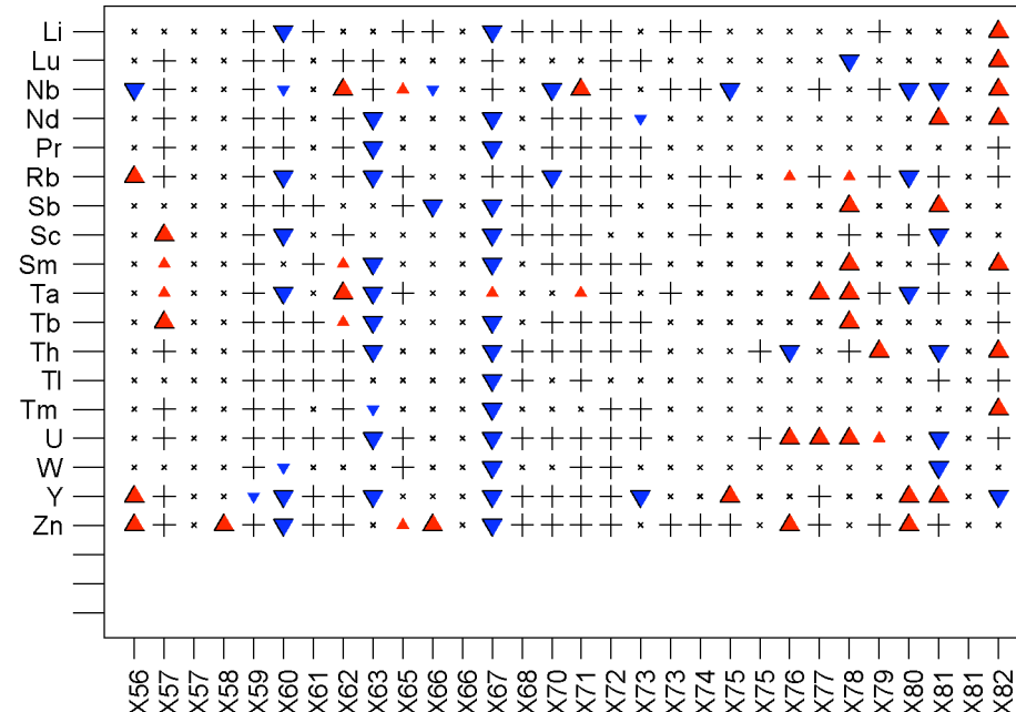
Figure 3b: GeoPT23 – Pegmatite OU-9. Multiple z-score charts for laboratories participating in the GeoPT23 round. Symbols indicate whether or not an elemental result complies with the -2 < z < +2 criteria. Satisfactory data are plotted as '+'. Data for other categories are plotted as follows: z < -3 (▽), -3 < z < -2 (▽), +2 < z < +3 (△), Z > +3 (△).
