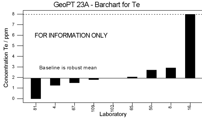
Figure 5b (cont'd): GeoPT23A – Manganese nodule, FeMn-1. Data distribution charts for information only for elements for which values could not be assigned.
