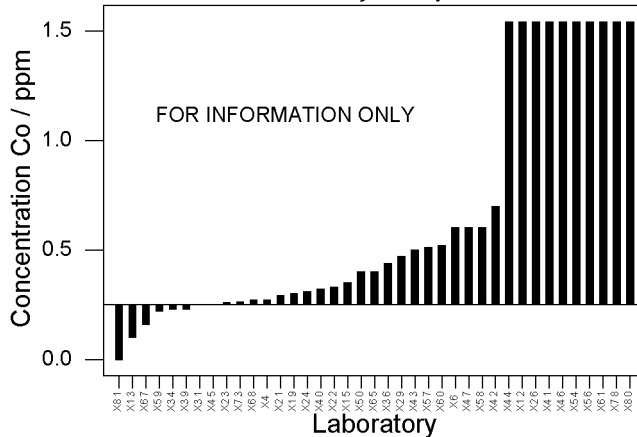
Figure 2: GeoPT23 – Separation Rapids Pegmatite, OU-9. Data distribution charts for information only for elements for which values could not be assigned.
