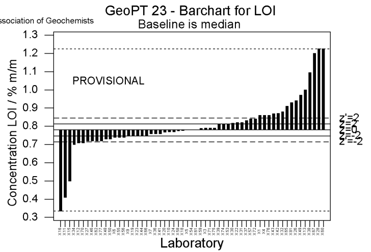
Figure 1: GeoPT23 – Separation Rapids Pegmatite, OU-9. Data distribution charts for elements for which values were assigned or provisional values given for guidance. Horizontal lines show the limits for -2 < z < 2 for pure geochemistry labs (solid lines) and -2 < z' < 2 for applied geochemistry labs (pecked lines).
