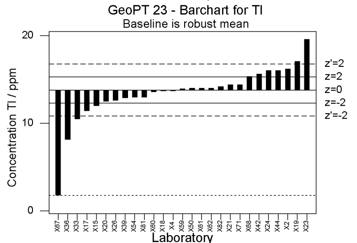
Figure 1: GeoPT23 – Pegmatite, OU-9. Data distribution charts for elements for which values were assigned or provisional values given for guidance. Horizontal lines show the limits for -2 < z < 2 for pure geochemistry labs (solid lines) and -2 < z' < 2 for applied geochemistry labs (pecked lines).
