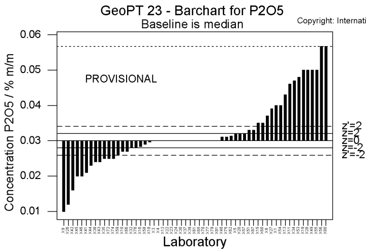
Figure 1: GeoPT23 – Separation Rapids Pegmatite, OU-9. Data distribution charts for elements for which values were assigned or provisional values given for guidance. Horizontal lines show the limits for -2 < z < 2 for pure geochemistry labs (solid lines) and -2 < z' < 2 for applied geochemistry labs (pecked lines).
