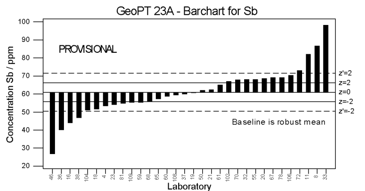
Figure 4b (cont'd): GeoPT23A – Manganese nodule, FeMn-1. Data distribution charts for elements for which values were assigned or provisional values given for guidance. Horizontal lines show the limits for -2 < z < 2 for pure geochemistry labs (solid lines) and -2 < z < 2 for applied geochemistry labs (pecked lines).
