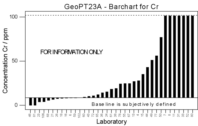
Figure 5b: GeoPT23A – Manganese nodule, FeMn-1. Data distribution charts for information only for elements for which values could not be assigned.
