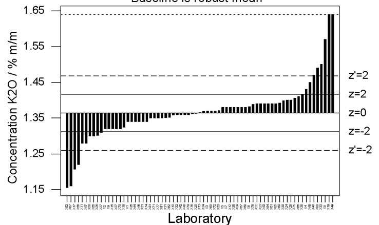
Figure 1: GeoPT23 – Pegmatite, OU-9. Data distribution charts for elements for which values were assigned or provisional values given for guidance. Horizontal lines show the limits for -2 < z < 2 for pure geochemistry labs (solid lines) and -2 < z' < 2 for applied geochemistry labs (pecked lines).
