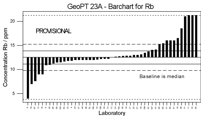
Figure 4b (cont'd): GeoPT23A – Manganese nodule, FeMn-1. Data distribution charts for elements for which values were assigned or provisional values given for guidance. Horizontal lines show the limits for -2 < z < 2 for pure geochemistry labs (solid lines) and -2 < z < 2 for applied geochemistry labs (pecked lines).
